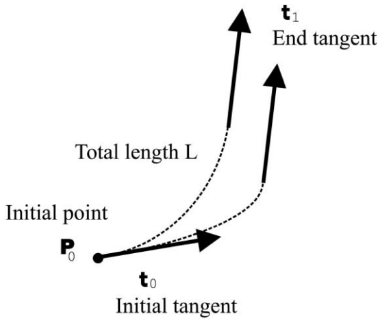
Fig. 3. Interpolation problem: finding a smooth curve whose initial point, tangent vectors at its initial and end points, and total length are given.
