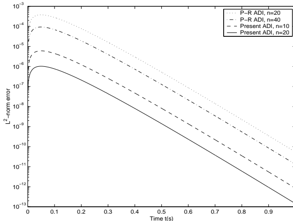
Figure 1: Comparison of the L^2 -norm errors produced by the present scheme and the P-R scheme at each time step.
