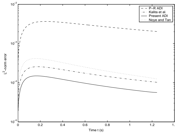
Figure 2: Comparison of the L^2 -norm errors produced by four different schemes at each time step.
